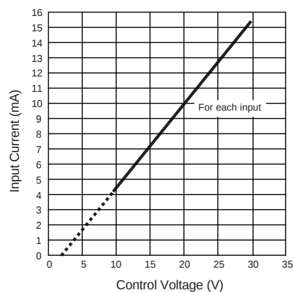
Figure 4c — SD48D50A2 relay
